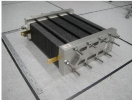
Development of PEMFC Stacks
