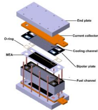
Development of PEMFC Stacks
