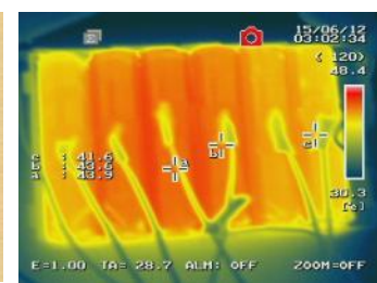
Thermal management of Li-battery
