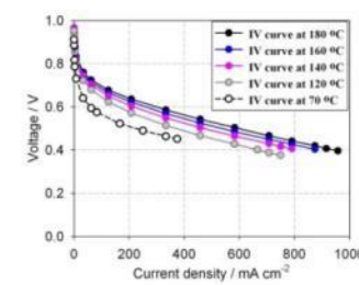
Fundamental studies on the high temperature PEMFC (120~180 °C)
